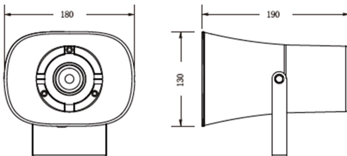
Figure 2: TI-HS7 Dimensions
